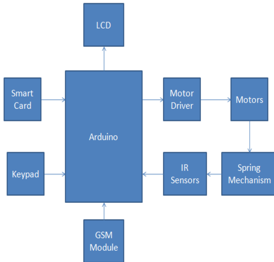
Fig 1 :block diagram
