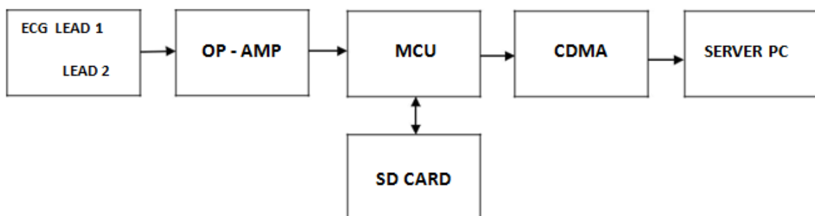
System architecture – ECG measuring system
