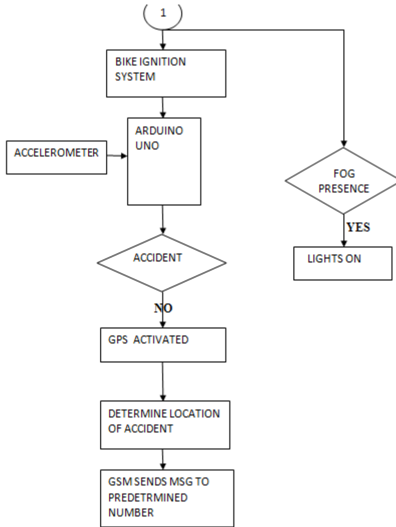
Fig 3: System flowchart
